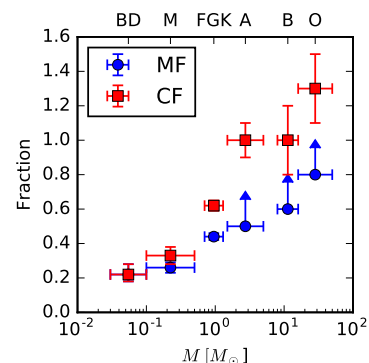
Figure 12.5: Multiple system fraction (blue) and companion fraction (red) versus primary star mass for field stars. Horizontal error bars show ranges of mass, and the upper axis shows the spectral type corresponding to that mass, with BD short for brown dwarf. Vertical error bars and limits indicate observational uncertainties. The multiple system fraction is the fraction of stars of that mass that are in multiple systems, while the companion fraction is the mean number of companions per star. The data plotted are taken from Table 1 of (Duchêne & Kraus, 2013).
