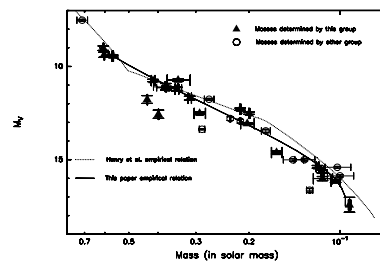
Figure 12.3: Empirically-measured mass-magnitude relationship in V band. Credit: Delfosse et al., A&A, 364, 217, 2000, reproduced with permission © ESO.
