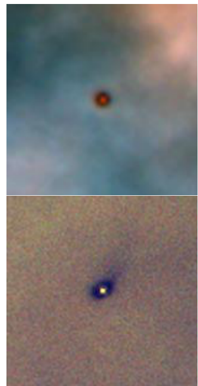
Figure 14.1: Two disks in the Orion Nebula seen in absorption against the nebula using the Hubble Space Telescope . Taken from http://hubblesite.org/newscenter/archive/releases/1995/45/image/g/ .
