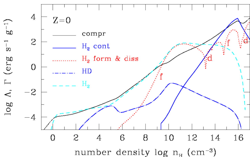
Figure 19.1: Results from a calculation of heating and cooling rates for processes operating in primordial gas of varying density, located at the center of a collapsing cloud. The processes included are heating by gravitational compression (black line), cooling by \text{H}_2 line (cyan) and continuum (solid blue) emission, cooling by HD emission (dot-dashed blue), and heating / cooling by collisional formation / dissociation of \text{H}_2 (dotted red). For each process, the value on the vertical axis indicates the rate of energy gain or loss per unit mass per unit time. Credit: Omukai et al. (2005), ©AAS. Reproduced with permission.
