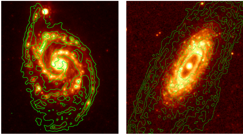
Figure 8.9: The galaxies NGC 5194 (left) and NGC 2841 (right), imaged in H I from the THINGS survey with the VLA, and 24 \mu m from Spitzer . Credit: Tamburro et al. (2008), ©AAS. Reproduced with permission.
