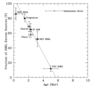
Figure 20.5: Fraction of stars that show near-infrared excess emission versus cluster age. The names of individual clusters are marked. Credit: Haisch et al. (2001), ©AAS. Reproduced with permission.
