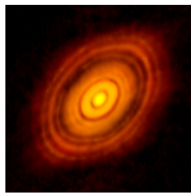
Figure 14.2: An image of the disk around the young star HL Tau made by the Atacama Large Millimeter Array (ALMA). The image shows dust continuum emission. Image from https://public.nrao.edu/static/pr/planet-formation-alma.html .
