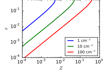
Figure B.8: x versus Z for n_{\text{H}} = 1, 10, and 100 \text{ cm}^{-3} .
