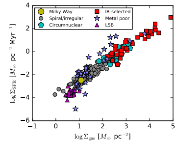
Figure 9.1: The observed collection between gas surface density \Sigma_{\text{gas}} and star formation surface density \Sigma_{\text{SFR}} , integrating over whole galaxies. Galaxy classes are as indicated in the legend; circumnuclear indicates circumnuclear starburst, IR-selected is galaxies selected based on their high-infrared luminosity, metal-poor is galaxies with substantially sub-solar metallicity, and LSB is low surface-brightness galaxies. Data from Kennicutt & Evans (2012).
