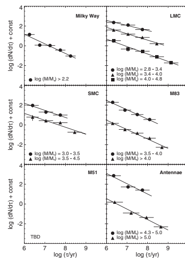
Figure 11.5: Measured distributions of star cluster ages in several galaxies. Clusters have been binned in mass, and different symbols show different mass bins, as indicated. Credit: Fall & Chandar (2012), ©AAS. Reproduced with permission.
