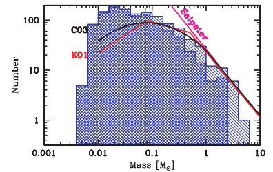
Figure 13.1: The IMF measured in a simulation of the collapse of a 500 M_{\odot} initially uniform density cloud. The single-hatched histogram shows all objects in the simulation, while the double-hatched one shows objects that have stopped accreting. Credit: Bate, 2009, MNRAS, 392, 590, reproduced by permission of Oxford University Press on behalf of the RAS.
