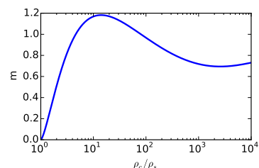
Figure B.3: Dimensionless mass m versus dimensionless density contrast \rho_c/\rho_s found by solving the isothermal Lane-Emden equation.
