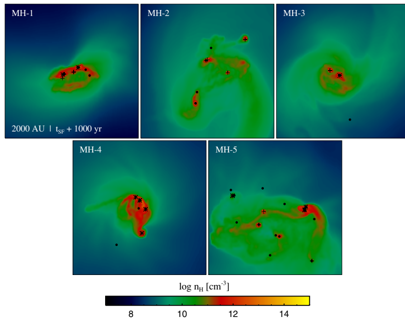
Figure 19.3: Results from a simulation of the formation of primordial stars. The images show the density in 2000 AU-sized regions in 5 different primordial halos, at a time 1000 years after formation of the first star in the simulation. Black dots, crosses, and stars indicate stars with masses < 1 M_{\odot} , 1 - 3 M_{\odot} , and > 3 M_{\odot} , respectively. Credit: Greif et al. (2011), ©AAS. Reproduced with permission.
