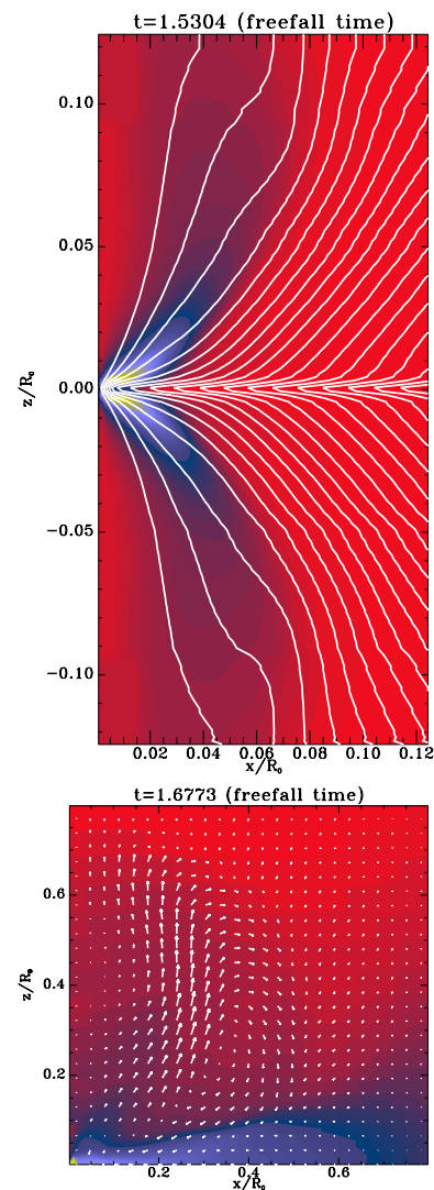
Figure 15.1: Results from a simulation of magnetized rotating collapse. The top panel shows the magnetic field structure; solid lines are poloidal magnetic field lines, while color indicates the azimuthally-averaged total magnetic field strength, on a scale from 0 – 3.5 mG. The bottom panel shows the density (color) and velocity (arrows) structure at a slightly later time in the simulation. The structure in the mid-plane is a non-rotating pseudo-disk. Credit: Hennebelle & Fromang, A&A , 477, 9, 2008, reproduced with permission © ESO.
