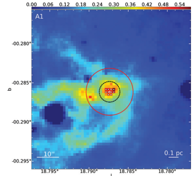
Figure 18.2: A massive protostellar core seen in IR absorption. Colors indicate the inferred column density in \text{g cm}^{-2} . Pixels marked with white dots are lower limits. The black circle shows a radius enclosing 60 M_{\odot} , and the red circle shows the core radius inferred by fitting a core plus envelope model to the azimuthally-averaged surface density distribution. Credit: Butler & Tan (2012), ©AAS. Reproduced with permission.
