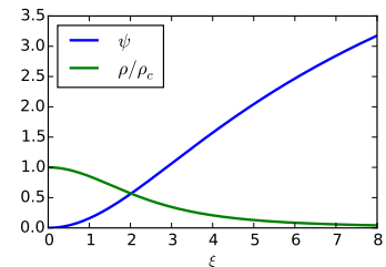
Figure B.2: Dimensionless potential \psi and density \rho/\rho_c = e^{-\psi} found by solving the isothermal Lane-Emden equation.
