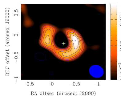
Figure 20.7: Dust continuum image of the disk around LkH \alpha 330, taken at 340 GHz by the SMA. Colors show the detected signal, and contours show the signal to noise ratio, starting from S/N of 3 and increasing by 1 thereafter. The green plus marks the location of the star. The blue circle is the SMA beam. Credit: Brown et al. (2008), ©AAS. Reproduced with permission.
