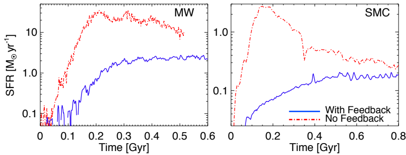
Figure 10.2: Star formation rates versus time measured in simulations of isolated galaxies performed with (blue) and without (red) a subgrid model for stellar feedback. One simulation shown is for a galaxy with properties chosen to be similar to the Milky Way (left), and one is for a galaxy chosen to resemble the Small Magellanic Cloud (right). Credit: Hopkins et al., 2011, MNRAS, 417, 950, reproduced by permission of Oxford University Press on behalf of the RAS.
